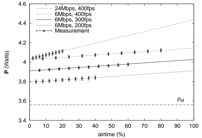
Fig. 6: Power consumed by (unacknowledged) reception versus airtime.
