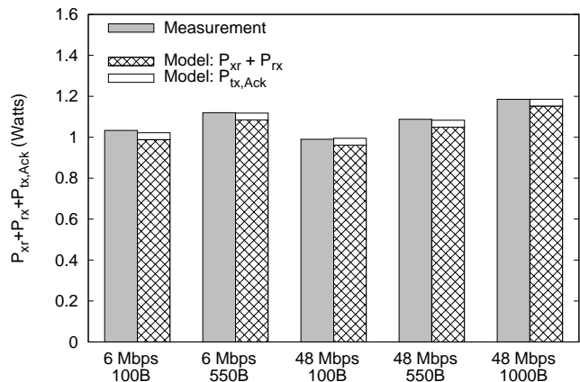
Fig. 7: Impact of sending ACKs on the receiver.
