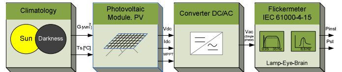
Figure. 1. Block diagram of the whole system.
