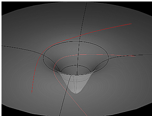
(a) Two geodesics (red) on a curved surface corresponding to a spherical gravitational field. Image taken from wikipedia.
