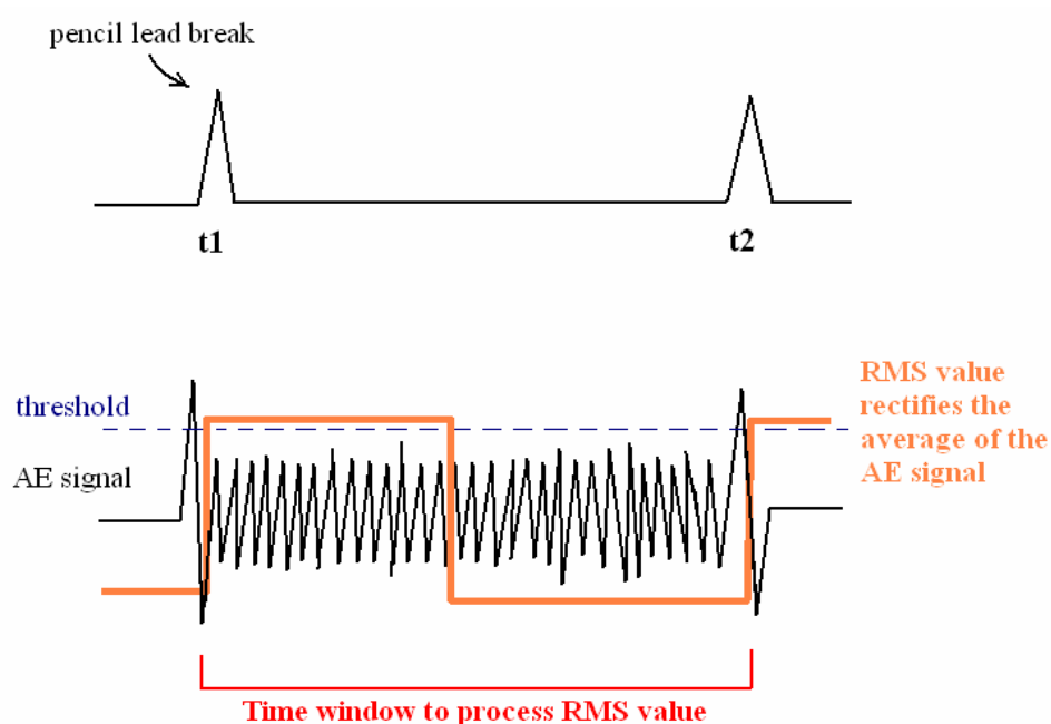
Figure 3.6- RMS function.
