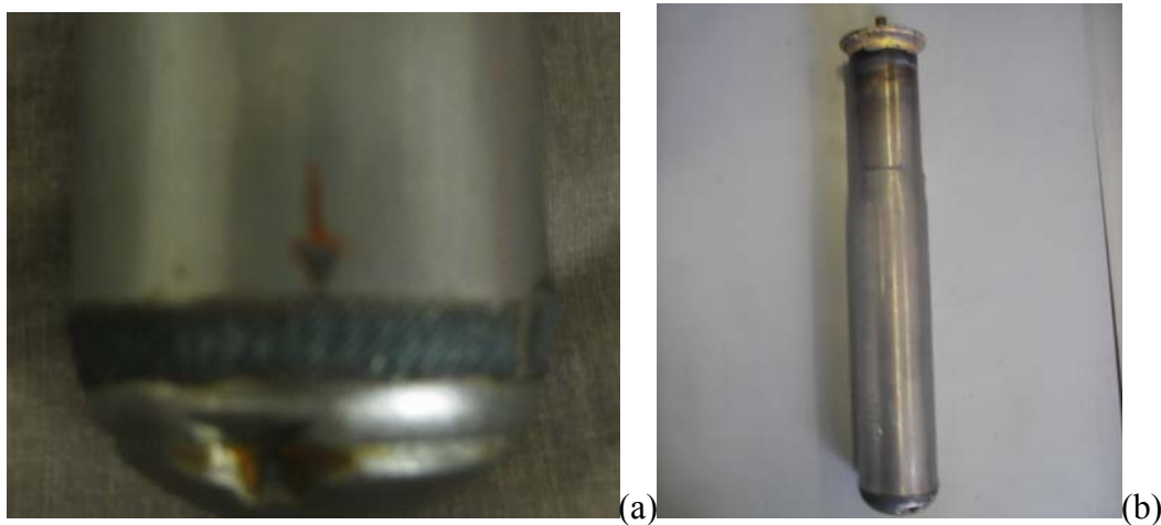
Figure 2.3- (a) Welding in which the leaks are difficult to observe. (b) Tube for shock absorber.
