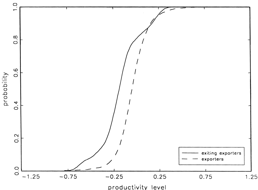
Fig. 4. Ex-ante productivity differences of exiting exporters versus continuing exporters: 1995–96 cohort of exiting firm (smooth sample distribution function).
