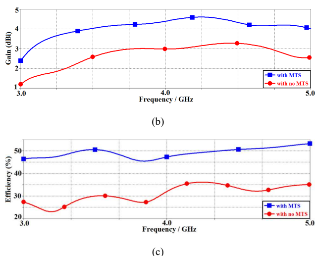
Fig.4. Simulated performance parameters of the 2-D periodic array of stacked non-metasurface sheets and metasurface sheets, (a), return-loss response, (b) radiation gain, and (c) radiation efficiency.
