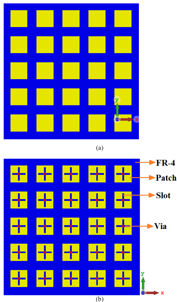
Fig.2. Metasurface sheet constructed from a 2-D periodic array of the square microstrip unit-cells, (a) basic structure without slot-line and via inclusions, and (b) with slot-line and via inclusions.
