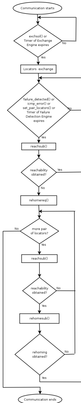
Fig. 8. Basic organizational chart of Multihoming Layer
