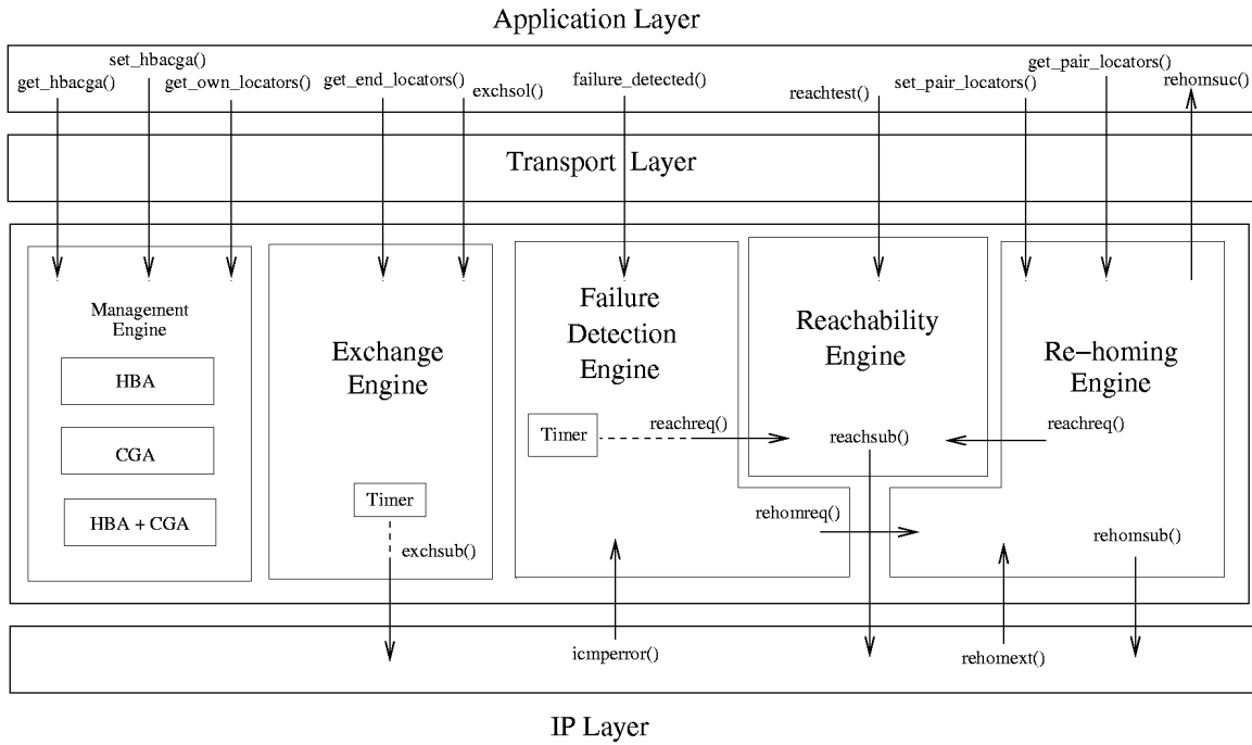
Fig. 4. Multihoming API Scheme
