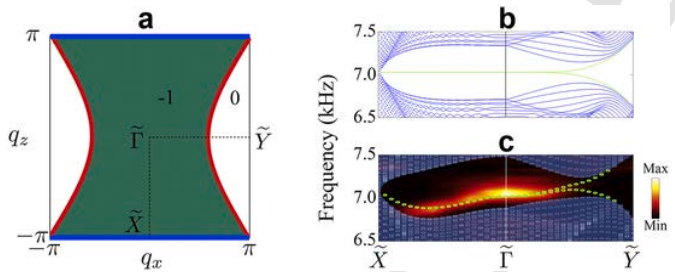
Fig. 4. Predicted and measured quasi-flat acoustic states. (a) Winding number \mathcal{W} surface mapping in momentum space, q_{||} = (q_x, q_z) . The green (white) region represents the area where \mathcal{W} = -1 ( \mathcal{W} = 0 ). The red and blue curves are the projections of nodal lines to the surface momentum space. (b) Theoretically obtained projected surface dispersions. The blue lines correspond to the bulk and the green ones to the surface states. (c) Measured (background intensity contour) and numerically simulated (shaded circles) projected bulk bands. The green dots highlight the surface waves dispersion. (For interpretation of the references to color in this figure legend, the reader is referred to the Web version of this article.)
