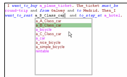
Figure 2. Example of an Ontology-guided Input
