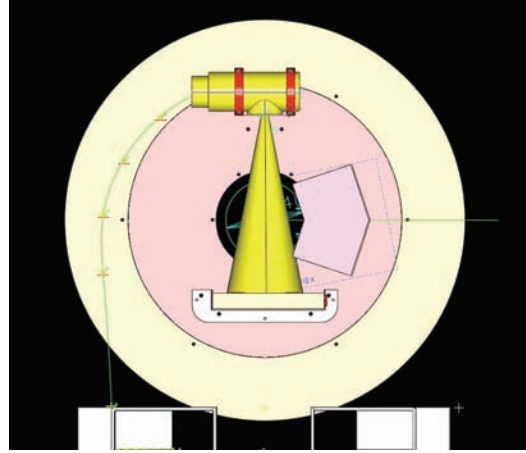
Figure 1: Layout of the PET/CT system showing the X-ray cone projected on the detector and one of the two PET detector boxes on the right of the cone beam.
