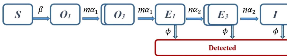
Fig. 1. Flow diagram of the compartmental stochastic SO^mE^nI (Susceptible, Occult, Exposed and Infectious) model with Erlang-distributed occult and exposed sojourn times (where m = n = 3 ), representing the dynamics of the bTB spread within the herd. Animals susceptible to M. bovis (S) become occult (O), infected but not detectable by SITT neither infectious, through the contact with shedding cattle at a rate \beta , the transmission coefficient. Occult
