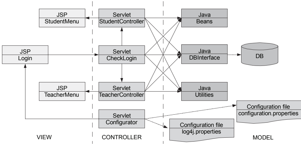
Figure 6. Architecture of EVAWEB v2
