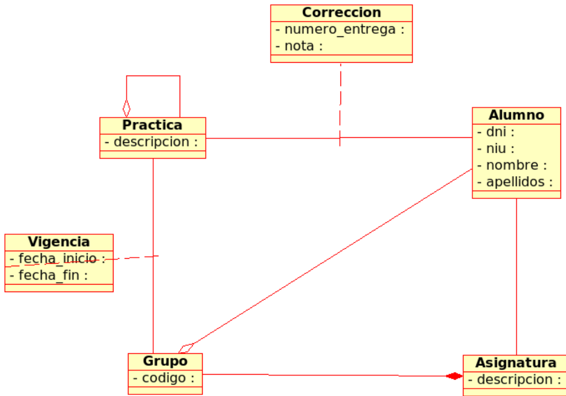
Class diagram
