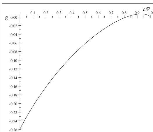
Figure 13: The function g evaluated at \frac{2}{5} \left[1 - \frac{c}{P}\right]
