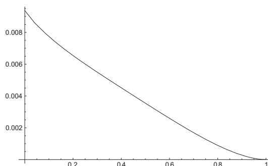
Figure 13: The function g evaluated at \frac{2}{5} \left[1 - \frac{c}{P}\right]
