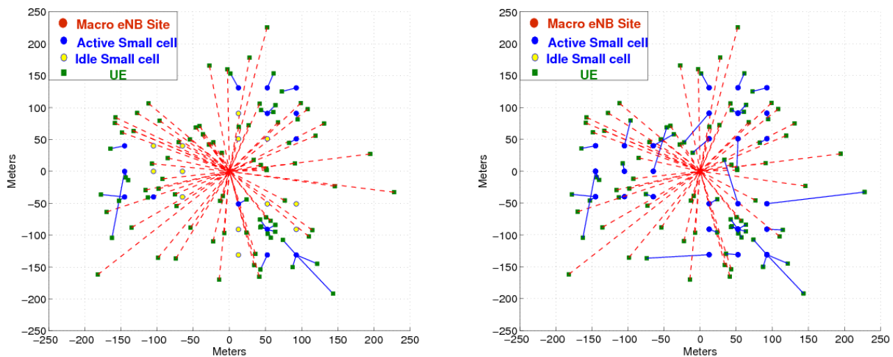
Figure 3: A snapshot of association pattern when using as association metric the strength of the downlink signal (left) and the aggregated network load (right).
