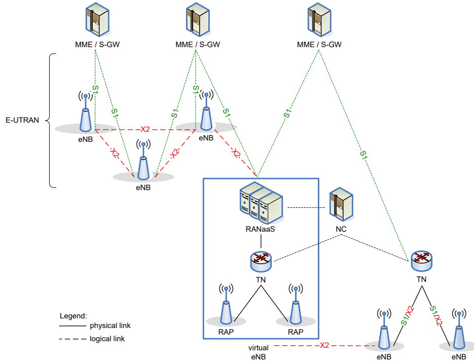
Figure 2: Architecture Evolution towards a 5G Mobile Network
