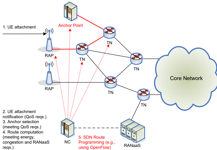
Figure 5: SDN-based Backhaul Management
