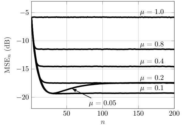
Fig. 2. MSE of the SNR estimates for different values of learning rate in time-varyant channels with f_D = 2 \cdot 10^{-3} .
