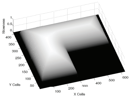
Fig. 3. The Fast Marching Method applied to a L-shaped environment gives: the slowness (velocity inverse) or repulsive potential and its associated vector field.
