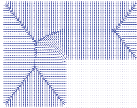
Fig. 3. The Fast Marching Method applied to a L-shaped environment gives: the slowness (velocity inverse) or repulsive potential and its associated vector field.
