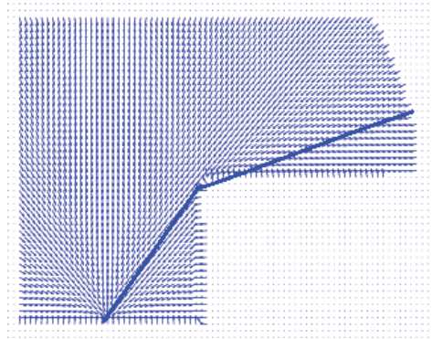
Fig. 2. Attractive potential, its associated vector field and a typical trajectory.
