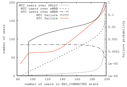
Fig. 12. Users in the system and failure probability of MTC with 1+3 repetitions and HTC think time of 100 ms (high HTC traffic)
