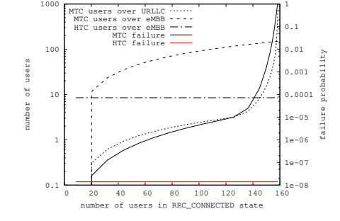
Fig. 10. Users in the system and failure probability of MTC with 2+2 repetitions and HTC think time of 20 ms (low HTC traffic)
