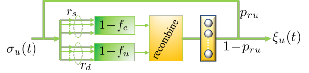
Fig. 2. Schematic representation of URLLC dynamics with packet repetitions over two sets of network slice resources. URLLC repetitions are recombined at the receiver and count as a single packet. The number of packets in a message is geometrically distributed, which is modeled with a probabilistic feedback. The infinite server after the recombine block models the inter-arrival time between packets.
