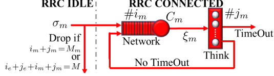
Fig. 3. Queuing network modeling the network processor for MTC
