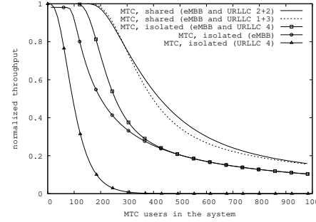
Fig. 9. MTC performance with a single slice ("MTC, shared") and with a stand-alone slice for each traffic type ("MTC, isolated").
