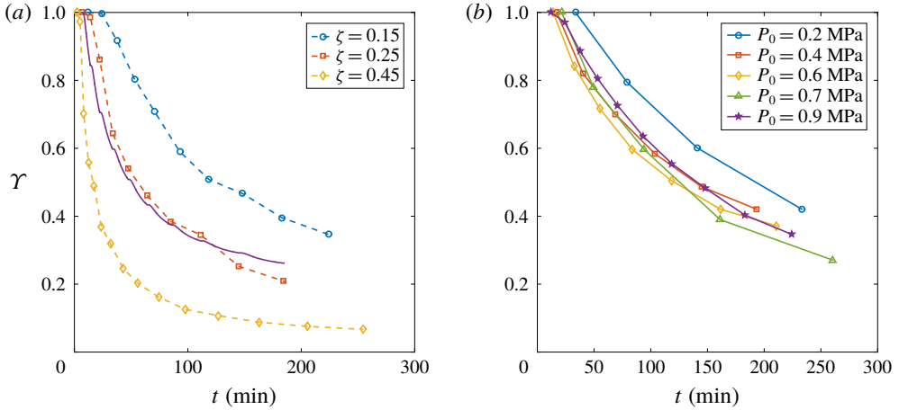
FIGURE 8. (Colour online) (a) Evolution of the depletion number \Upsilon in time with different supersaturation level \zeta and fixed P_0 = 0.9 MPa. An evident faster depletion occurs with larger \zeta . The solid line stands for the theoretical behaviour by Moreno Soto et al. (2017) with \alpha = 0.42 for the case \zeta = 0.25 . (b) Evolution of \Upsilon in time for different starting saturation pressure P_0 and \zeta = 0.15 . The experimental results make it reasonable to suggest that P_0 , and therefore the intensity of the transition to convection, plays a secondary role in the speed of depletion.
