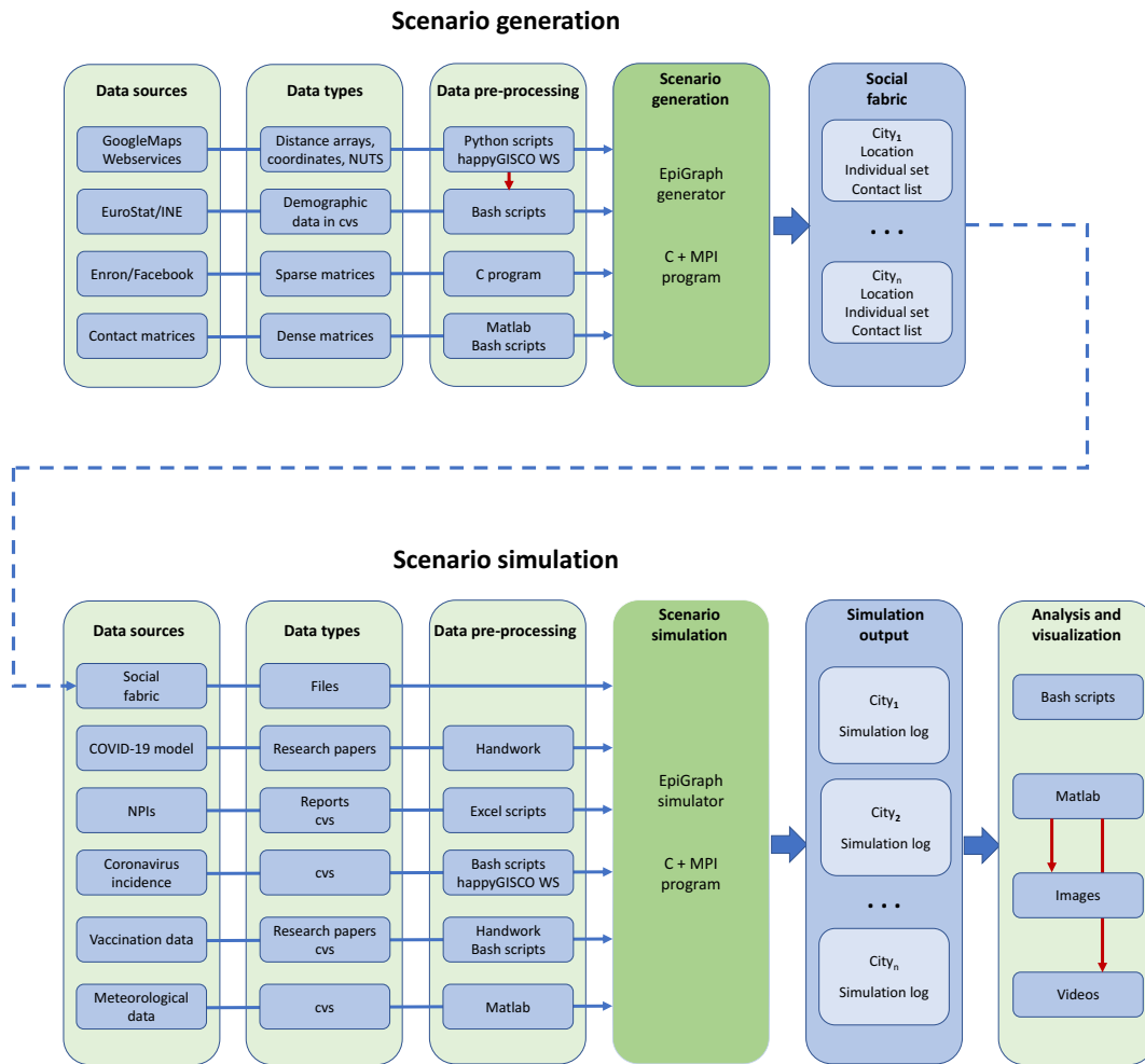
Fig. 2: Overview of the data flow related to EpiGraph simulation. In the scenario generation stage (upper part figure) the the social fabric is generated and stored in files. In a second stage this information is used in combination with other sources of data (lower part figure) to perform the simulation.
