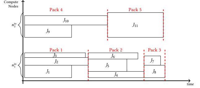
(a) The mapping of 11 applications into packs
