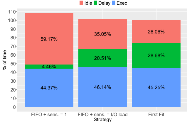
Figure 13: Average execution, idle and delay time (normalized) for different strategies
