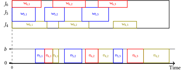
(b) The scheduling of I/O operations (bottom) within Pack 2. Computations are allocated on dedicated compute nodes and can start as soon as the I/O is transferred, but I/O operation share the available bandwidth b and can delay applications.
