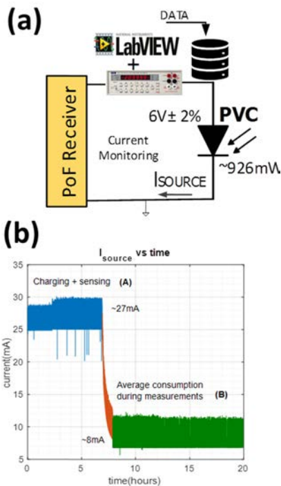
Fig. 4. (a) Experimental setup to characterize the smart remote node power demand. (b) Smart remote node electrical current demand depending on its operation mode.
