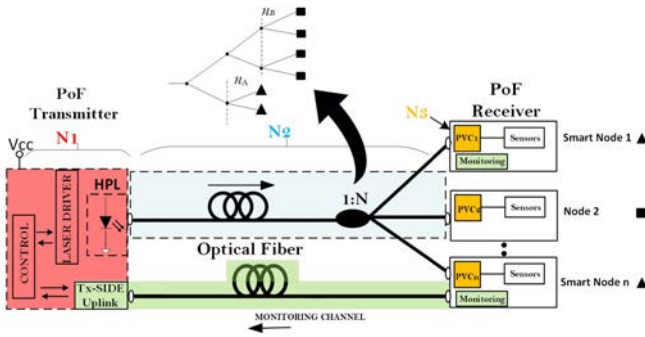
Fig. 1. Schematic of the generic PoF topology addressing N remote sensor nodes. HPL: High Power Laser. PVC: Photovoltaic converter. Some smart nodes ( \blacktriangle ) with monitoring capabilities are shown. Inset: asymmetric topology.
