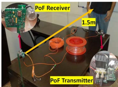
Fig. 5. Picture of the PoF system experiments carried out to feed a smart node that includes a temperature/presence sensor, a flame detector, microcontroller-based control electronics, an energy manager and an upstream optical data channel.
