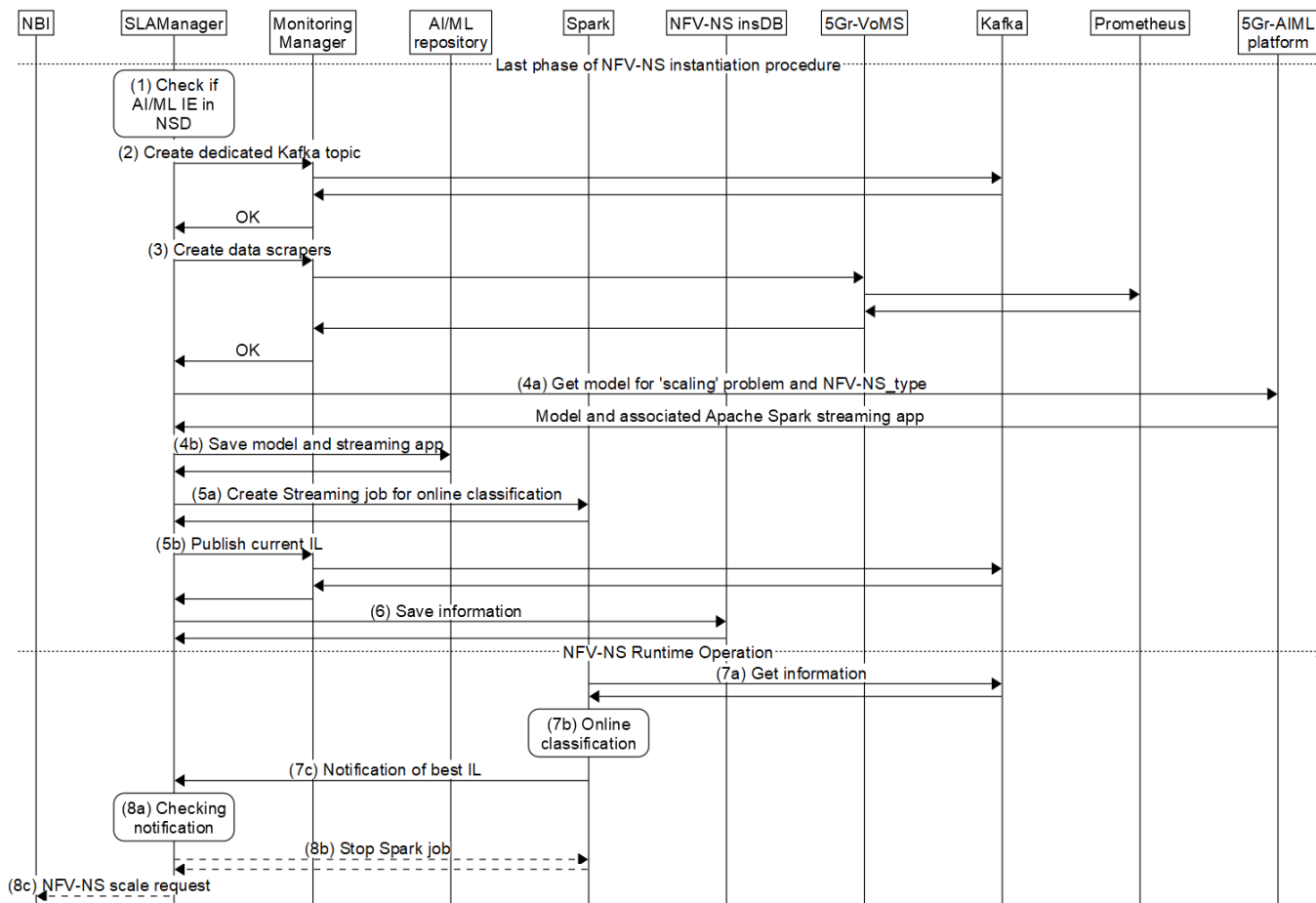
Fig. 2: 5Growth workflow to configure AI/ML-based scaling operation
