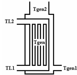
Figure 9: Schematic representation of the generator of the Yazaki WFC10.
