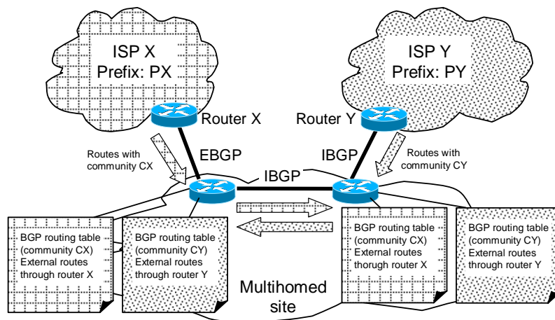
Figure 6. SAD routing deployment using BGP communities
