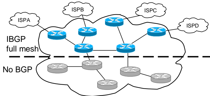
Figure 5. IBGP full mesh
