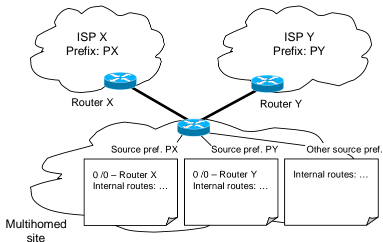
Figure 3. SAD routing
