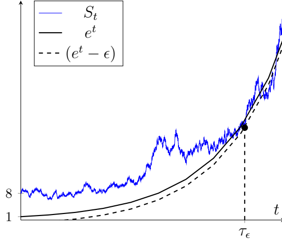
Figure 1: An example of realization of the stopping time \tau_\epsilon defined in (4.9).
