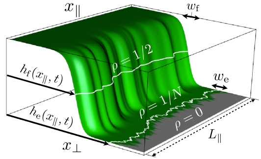
FIG. 1 (color online). FKPP front in d_E = 3 , as obtained by numerical simulations of Eq. (2), with indication of notation and quantities introduced in the text. White lines correspond to equipotential lines at \rho = 1/2 (front interface) and \rho = 1/N (edge interface).
