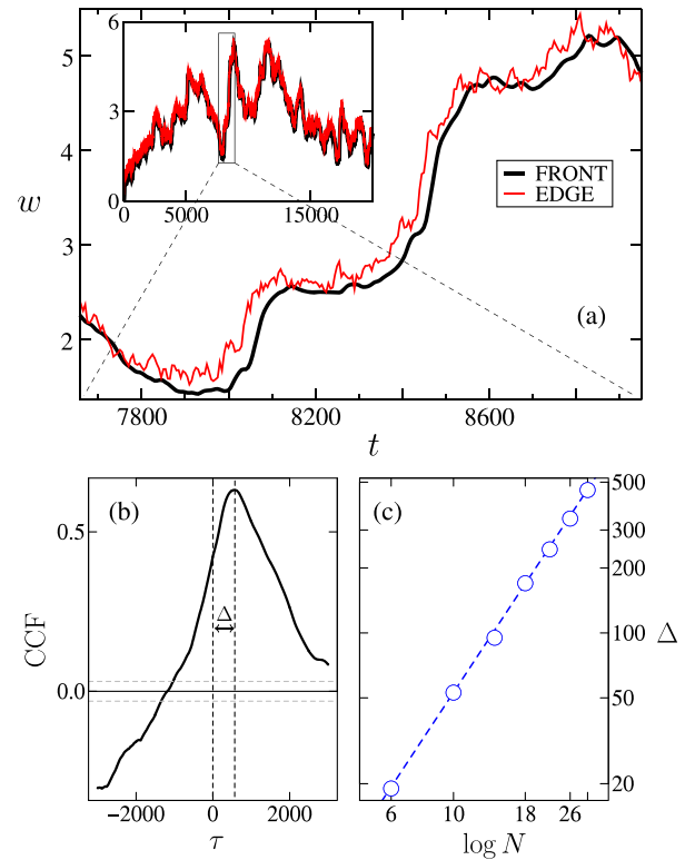
FIG. 3 (color online). (a) Roughness time series for the edge (thin red solid line) and front (thick black solid line) interfaces, for a single noise realization. Inset: Full dynamics. (b) Cross-correlation function between front and edge roughness time series, for a single noise realization and N = 10^{30} . The time to the first maximum defines the lag \Delta ; see main text. (c) Values of \Delta (circles) for different values of N , and L_y = 512 . The line is a fit to \Delta \sim \log^\gamma N , where \gamma = 1.97 . Statistical errors are smaller than the symbol size. All units are arbitrary.
