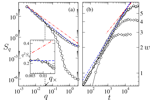
FIG. 2 (color online). (a) Structure factor of the front (circles) and edge (diamonds) interfaces, together with the behavior of the 1D (blue dashed) and 2D (red dot-dashed, asymptotic) KPZ behaviors. System size is L_{\parallel} = 1024 . Inset: rescaled structure factor q^2 S_q as a function of q . For small q , the front and edge interfaces both show 1D KPZ behavior S_q \sim q^{-2} . Lines correspond to those in the main panel. (b) Time evolution of the roughness of the edge interface for L_{\parallel} = 2048, 1024 , and 512 (diamonds, top to bottom) and roughness of the front interface for L_{\parallel} = 2048 (circles) compared to the 1D (blue dashed) and 2D (red dot-dashed) KPZ scaling behavior. In all cases N = 10^6 . Solid lines are guides to the eye. All units are arbitrary.
