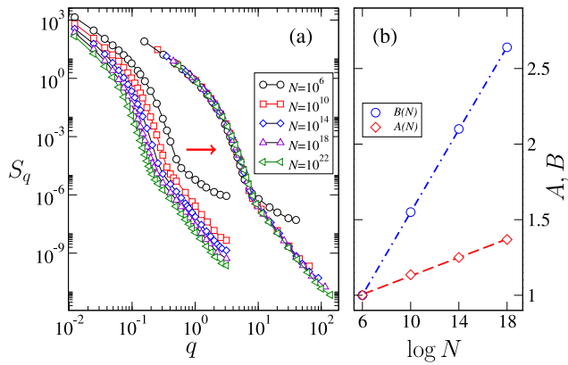
FIG. 4 (color online). (a) Structure factor of the front interface for different values of N , together with rescaled curves obtained by collapsing all curves to the N = 10^6 data in the macroscopic region q \ll 1 ; see main text for details. (b) Rescaling factors of S_q and q as functions of N (symbols) together with linear fits (lines). Statistical errors are smaller than the symbol size. All units are arbitrary.
