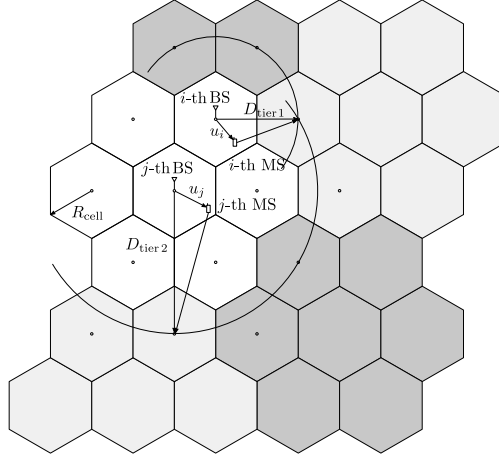
Figure 4.1: System layout with clusters of seven cells of radius R_{\text{cell}} (the radius of the circle circumscribing the cell) with an example of two users, with the distances D_{\text{tier 1}} and D_{\text{tier 2}} , respectively, from their BS to the interfering BSs.
