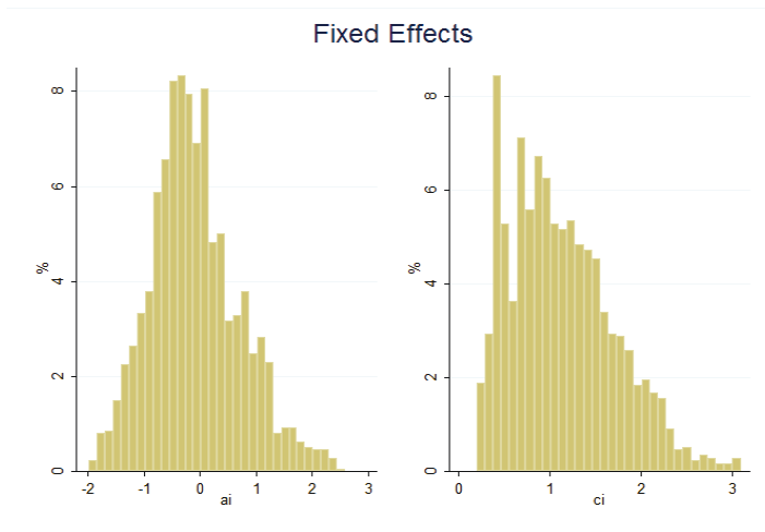
Figure 1: Density estimate (histogram) of the fixed effects from MMLE.
