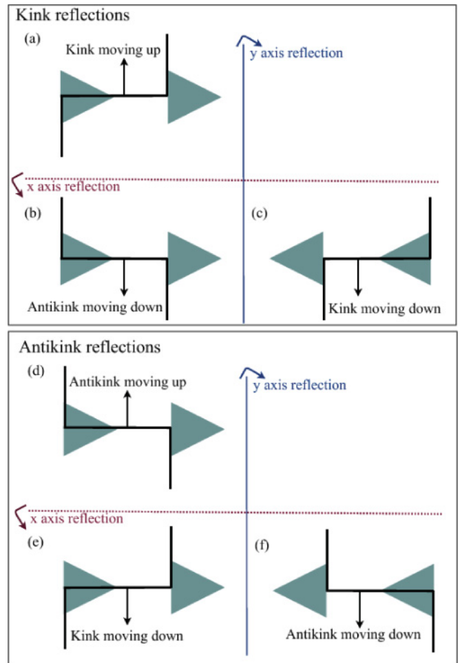
FIG. 6. (Color online) Broken symmetry in a 2D kinked wall. (a) Kink moving upward. (b) After an x-axis reflection an antikink moving downward is obtained. (c) After a second y-axis reflection a kink moving downward on a different array (inverted triangle array) is obtained. From (d) to (f) the same reflections are shown for an antikink.
