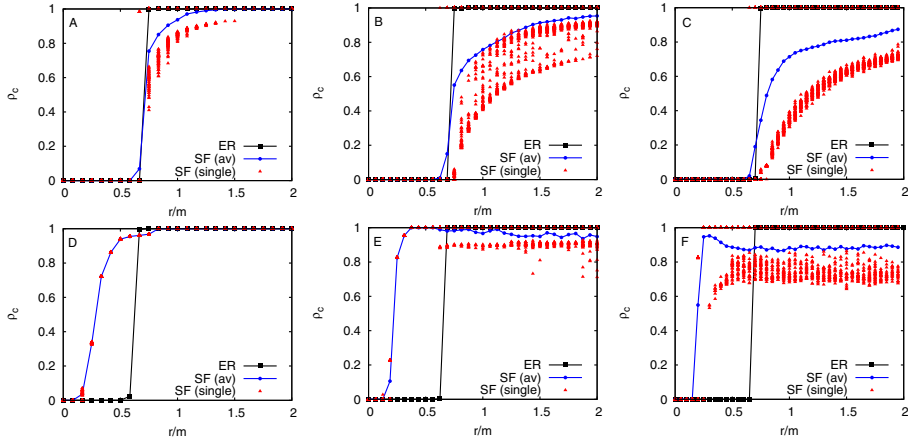
Fig. 3: (Colour on-line) Average fraction of cooperators, \rho_c , as a function of the normalized enhancement factor r/m (we have fixed z = 1 ). Panels (A), (B) and (C) (top) are for the FCG formulation of the PGG, while (D), (E) and (F) (bottom) are for its FCI version. The panels correspond to m = 3 ((A) and (D)), m = 4 ((B) and (E)) and m = 5 ((C) and (F)). The curves with filled squares correspond to ER networks, while the results for the SF ones correspond to the curves with filled circles. The triangles account for the level of cooperators reached in each of the 10^2 realizations performed on SF networks for each value of r/m .
