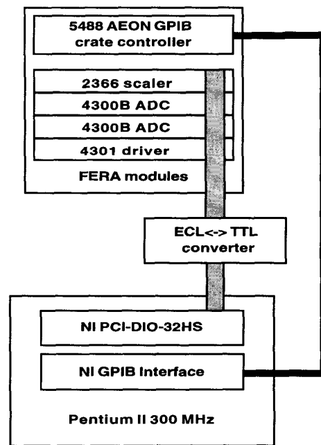
Figure 1. System schematics.
