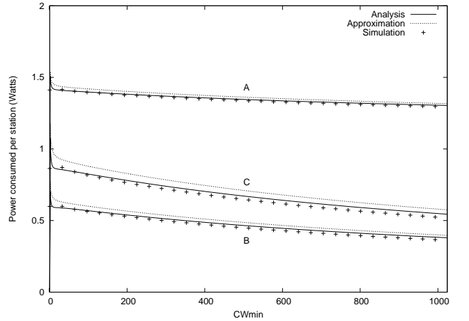
Fig. 2. Power consumption for the energy profiles of Table I for different CW configurations, N = 10 .
