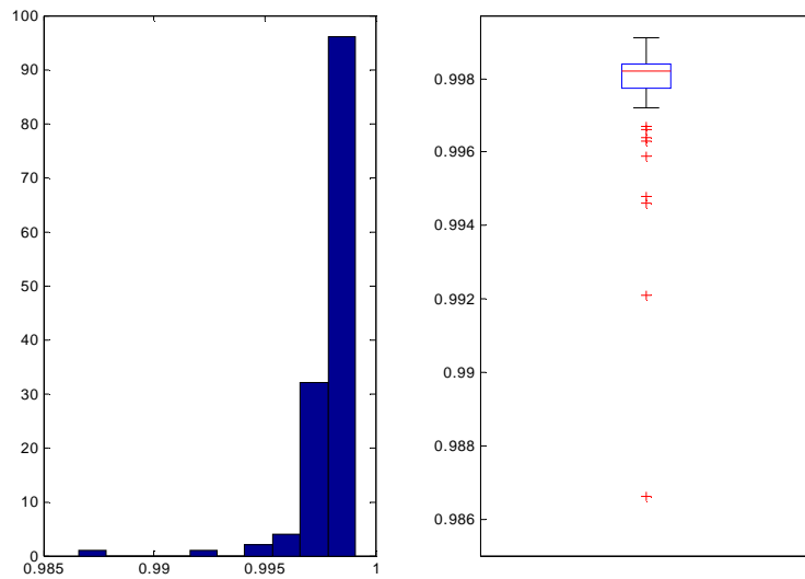
Graph 5: Distribution of the largest Box-Tiao canonical eigenvalue
