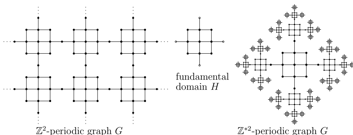
FIGURE 6. An example with a covering group having two generators. The fundamental domain has 13 vertices and four boundary vertices. On the left, the covering graph with Abelian group is plotted. In this case, the symmetrised KD spectrum \hat{J} already give the spectrum of the covering operator. On the right, we have a \Gamma -covering with \Gamma = \mathbb{Z}^{*2} = \mathbb{Z} * \mathbb{Z} , the free (non-abelian) group with two generators. Here, we only have the spectral estimate \sigma(\check{\Delta}_{G^*}) \subset \hat{J} .
