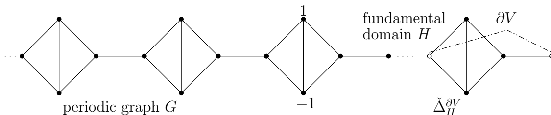
FIGURE 4. A non-bipartite graph. The related spectral information of this graph is visualised in Figure 2. The Laplacian on H without Dirichlet conditions is not plotted here. The two values \pm 1 at the vertices indicate the eigenfunction associated to the eigenvalue \lambda_3 = 4/3 , independent of \vartheta ; the other vertex values being 0.
