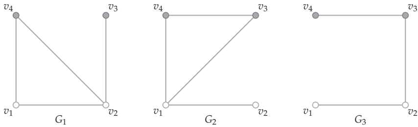
Figure 1. The set \{v_3, v_4\} is a simultaneous local metric basis of \{G_1, G_2, G_3\} . Thus, Sd_I(G_1, G_2, G_3) = 2 .
