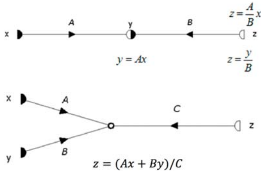
Figure 1. Elementary graph-algebra operations.
