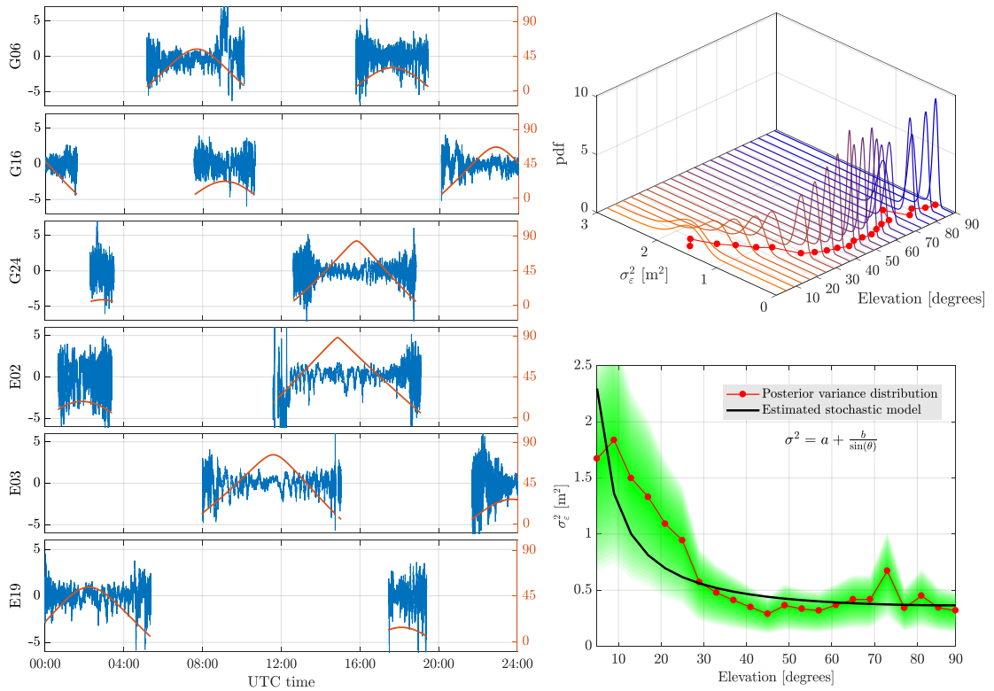
Figure 7: On the left, time series of the CMC combination for the day 42 of the year 2018, collected at the Mecklenburg-Vorpommern vessel. A total of six satellites, three from GPS and three from Galileo is shown. On the right, the inferred IG based distributions for the noise variance conditioned on the satellite elevation for GPS L1 observations. On the top right, the inferred IG based distributions for the noise variance conditioned on the satellite elevation for GPS L1 observations. On the bottom right, the satellite-based stochastic model for the multipath and receiver noise is regressed from the mode of the aforementioned IG distributions. In our study, we have observed that three days of data collection are sufficient to obtain congruent results regardless of the bin sizes.
