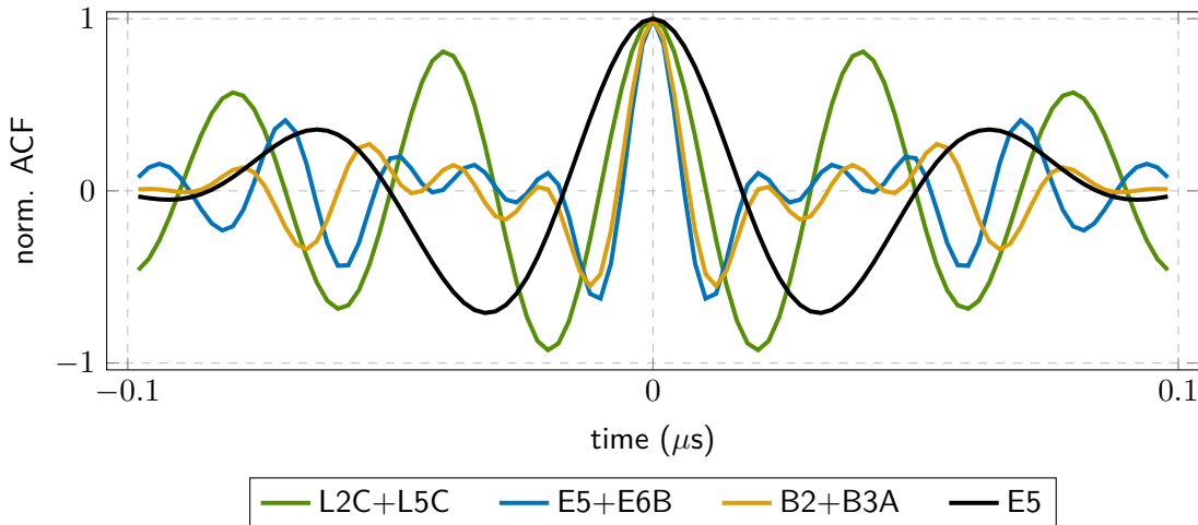
Figure 1.9: Comparison of the main normalized ACF peaks for a set of meta-signals: L2C+L5C, E5+E6B and B2+B3. For completeness, Galileo E5 is show in black.
