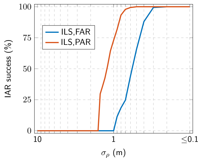
Figure 2.11: Experimental success ratio for the FAR and PAR integer estimation against the standard deviation of the undifferenced code observations' noise for the low noise and threshold regimes.
