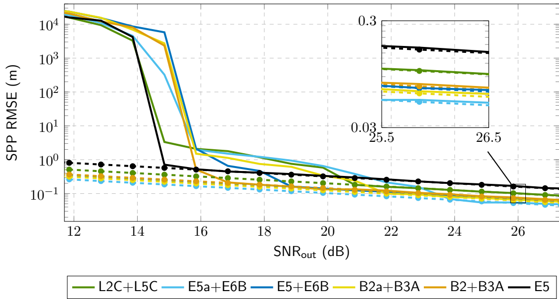
Figure 1.12: SPP position CRB (dashed lines) and associated RMSE (solid lines) versus \text{SNR}_{\text{out}} for a selection of meta-signals. For completeness, Galileo E5 is shown in black.
