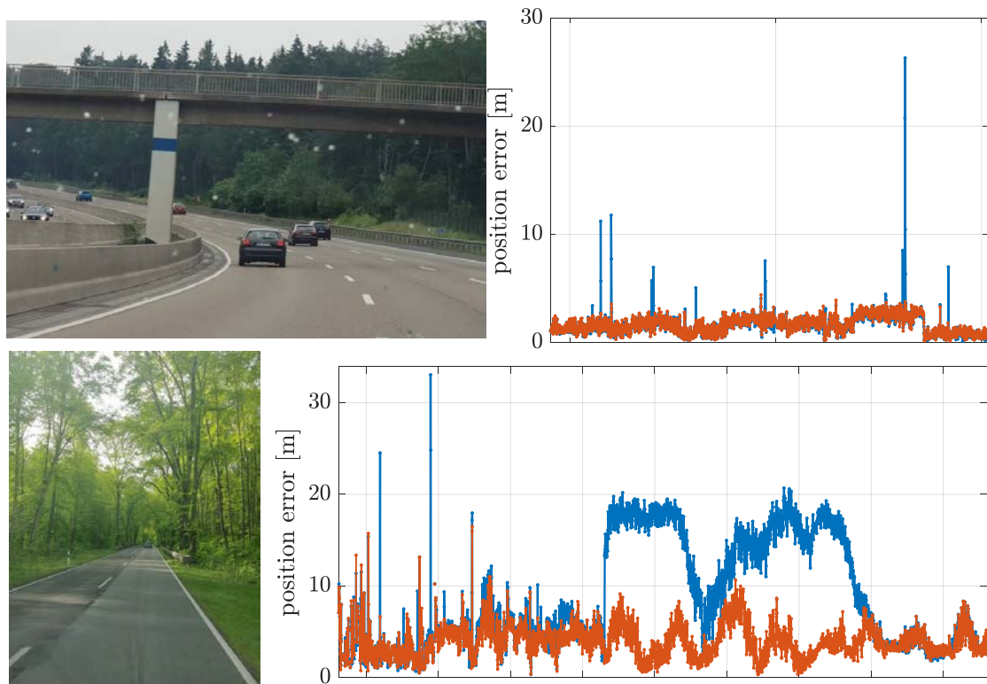
Figure 5.10: Detail on the time spans A and B for the measurement campaign. The first row (time span A) corresponds to bridge passing during highway navigation, while the second row (time span B) occurs during national road navigation under tree foliage. The pictures on the left were taken from the vehicle during the measurement campaigns, while the figures on the right depict the norm of positioning errors over time.
