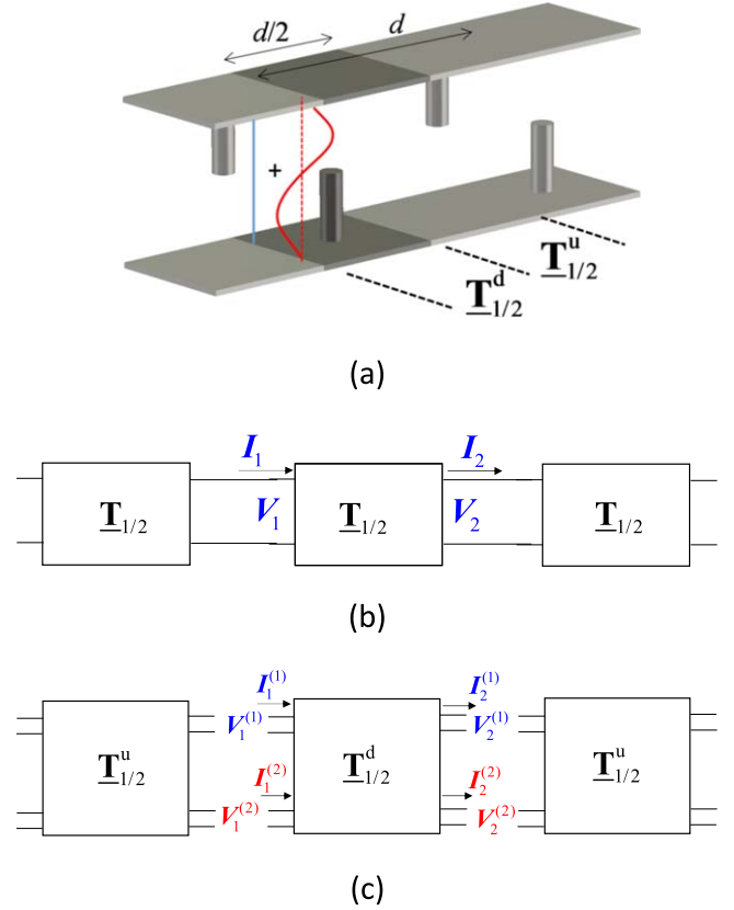
Figure 18. (a) 1D glide-symmetric pin-based metasurfaces. (b) Model retaining only one mode at each port ( \mathbf{T}_{1/2}^d = \mathbf{T}_{1/2}^u = \mathbf{T}_{1/2} ). (c) Model retaining two modes.
