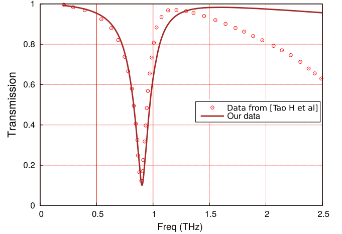
Figure 24. Transmission for the metasurface made up of split ring resonators already studied in [187].
