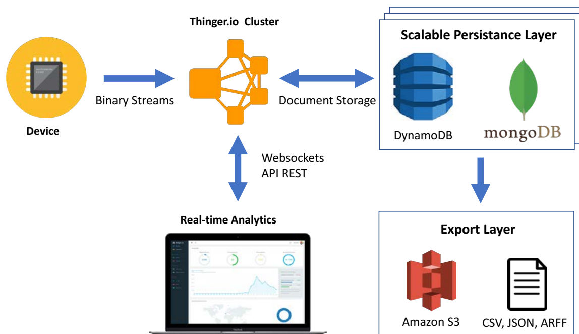
Figure 7. Thingier.io Big Data Storage Overview.
