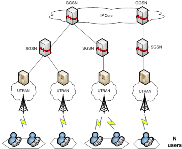
Figure 6: Network model
