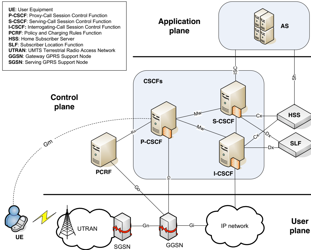
Figure 1: IMS architecture
