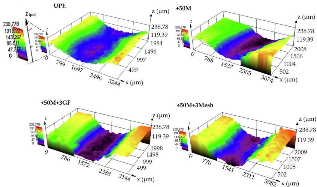
Fig. 10 – 3D images by optical microscopic for UPE matrix and bio-composites. Z-axis is the same for all 3D images; it is enlarged on the UPE image.
