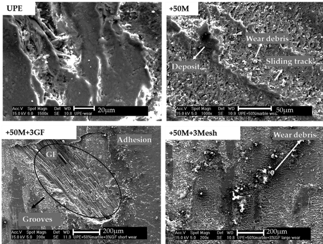
Fig. 11 – Wear track micrographs by SEM for the UPE and bio-composites.
