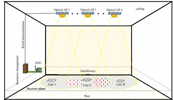
FIGURE 1. Diagram of an indoor hybrid VLC/WiFi network.
