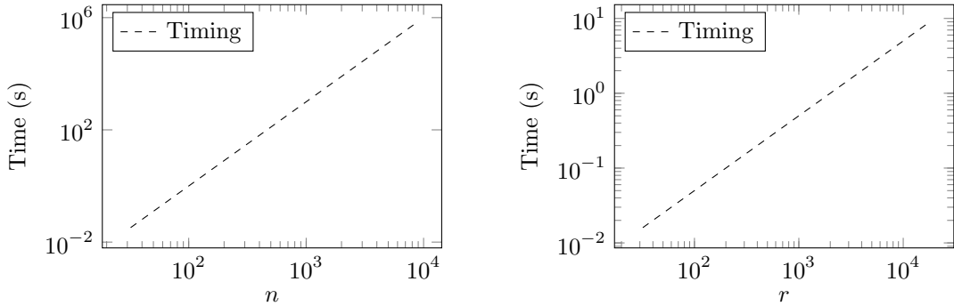
Figure 1: On the left, the CPU time required by the algorithm described in Section 8.6 for the \star = \mathsf{T} case, as a function of n . The timings reported are for a system with 3 equations, already in the required triangular form. The problems tested have sizes ranging from n = 32 to n = 8192 . On the right, the CPU time required by the algorithm described in Section 8.6 for the \star = \mathsf{T} case, as a function of r . The timings reported are for a system with r equations and coefficients of size 16 \times 16 , already in the required triangular form. The problems tested have sizes ranging from r = 32 to r = 16384 .
