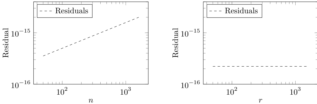
Figure 2: On the left, average residuals of 100 systems of \mathsf{T} -Sylvester equations solved via the algorithm described in Section 8. The systems considered have 3 equations with a variable coefficient size n . On the right, average residuals of 100 systems of \mathsf{T} -Sylvester equations solved via the algorithm described in Section 8. The systems considered have coefficients with size 8 \times 8 , and r equations.
