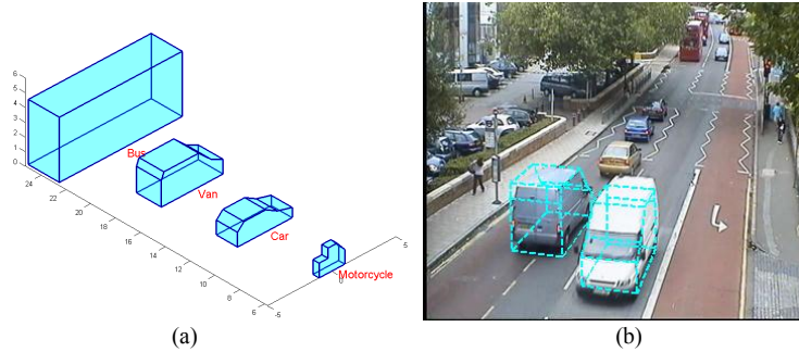
Fig. 6. 3D wireframe models [17] with true size (a) and samples of their projections on the ground plane (b).
