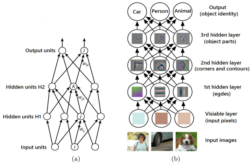
Fig. 7 (a) Illustration of a multilayer network model [115]. This model allows a computer to automatically determine the representations needed for prediction tasks. The first layer (input units) is called “ visible layer ”, it contains natural data in their raw form (e.g., a collection of pixels values). Starting from the visible layer, a series of hidden layers is built through extracting increasingly abstract features from lower levels. In other words, more abstract concepts are learned from the lower levels. The highest layer contains useful information for exploring and predicting the content of input data. (b) An example of a deep learning model for classification problems [256, 59]. Given some pictures, the first layer includes an array of pixel values. The first hidden layer represents the presence of edges. Then, the second hidden layer can identify corners and contours from edges in the first layer. By connecting corners and contours, the third layer can determine specific objects.
