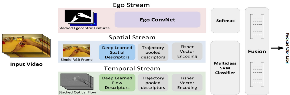
Fig. 18 Three-stream CNN architecture for the recognition of wearer’s actions proposed by Singh et al. [186].
