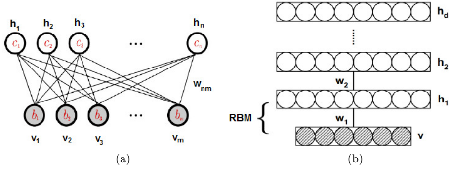
Fig. 14 (a) An example of a RBM with m visible units and n hidden units. (b) The schematic overview of a deep belief networks composed of d RBMs. W_1, W_2, \dots, W_h are the weights matrices between the connections.
