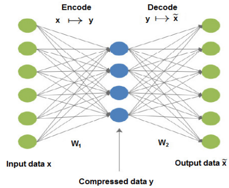
Fig. 15 The typical structure of an autoencoder.
