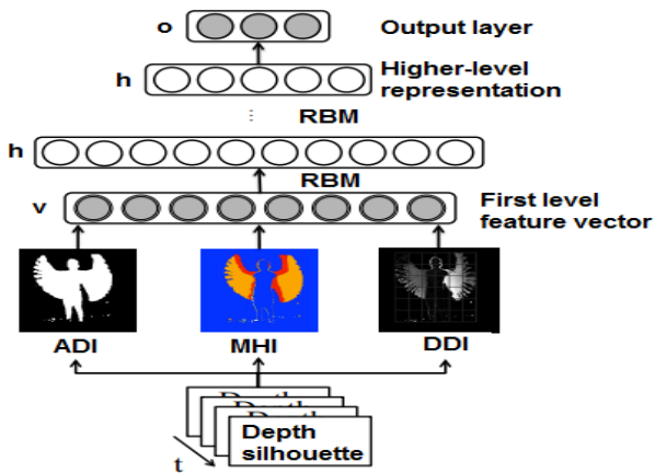
Fig. 25 An overview of the DBN architecture for human action recognition proposed by Foggia et al. [52]. Three derived images (ADI, MHI, DDI) are computed from depth images and feed into the first level of the network. A more abstract representation is obtained at higher level. Finally, the classification is done using a feed-forward neural network.
