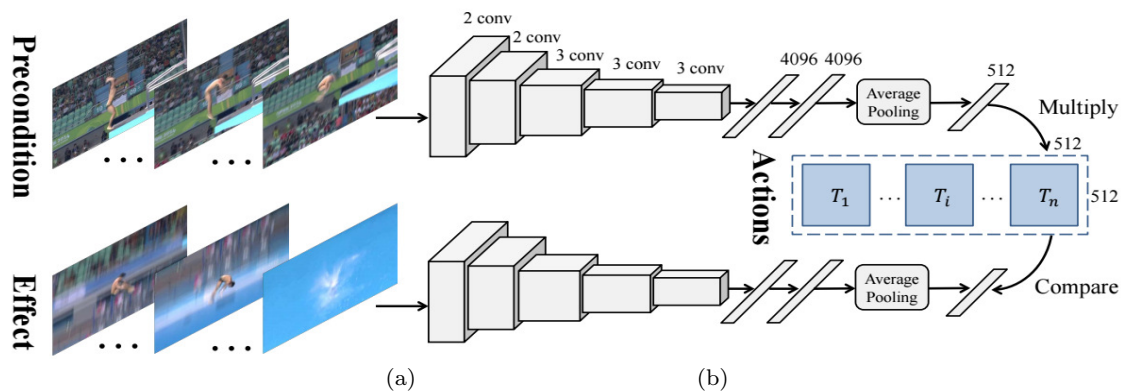
Fig. 19 The Siamese network architecture proposed by Wang et al. [237].
