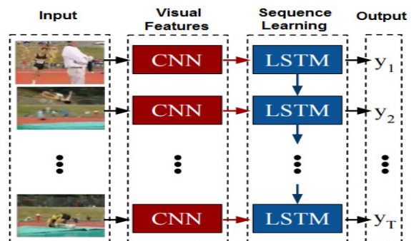
Fig. 22 DL framework combining CNN and RNN-LSTM for action recognition proposed by Donahue et al. [43]
