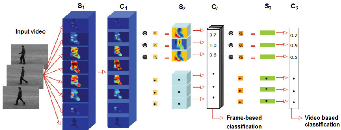
Fig. 16 The framework for recognizing human action proposed by Jhuang et al. [90]. Given a gray-value video sequence as input data, the S_1 stage locates the object in image frame by using spatio-temporal filters. Each C_1 unit is computed by applying a local max over for each S_1 unit for down-sampling. From the C_1 stage, we perform a template matching operation for identifying intermediate-level features of the model. The C_2 stage is constructed by computing the global max over each S_2 unit. The high-level features are extracted in S_3 through a template matching and the C_3 features are computed from S_3 using the same way like computing C_2 . The last stage is a linear multiclass SVM classifier that is able to recognize the actions using the C_3 features as input.
