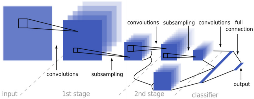
Fig. 9 Illustration of the typical block diagram of a CNN [176].
