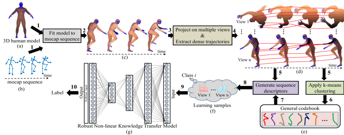
Fig. 26 Architecture of R-NKTM and its learning process [158]. Firstly, 3D human models are fitted to real motion capture data for generating realistic 3D videos. These 3D videos are then projected on 2D planes for calculating dense trajectories. A general codebook is learned from trajectories which is then used as the input of R-NKTM. By this way, the R-NKTM can learn features of human action videos and use it for testing process.
