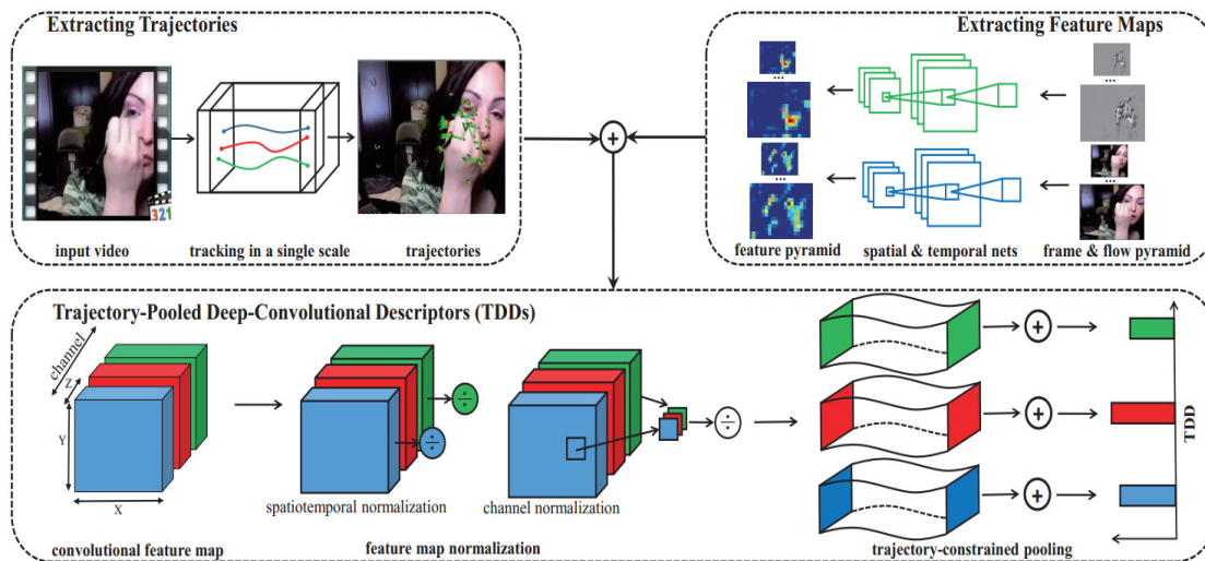
Fig. 21 The framework for action recognition proposed by Wang et al. [229]. Given an input video, the model extracts trajectories. Multiscale convolutional feature maps are extracted by a CNN at the same time. Trajectory Pooled deep-Convolutional Descriptors (TDDs) are then estimated from a set of improved trajectories and convolutional feature maps.
