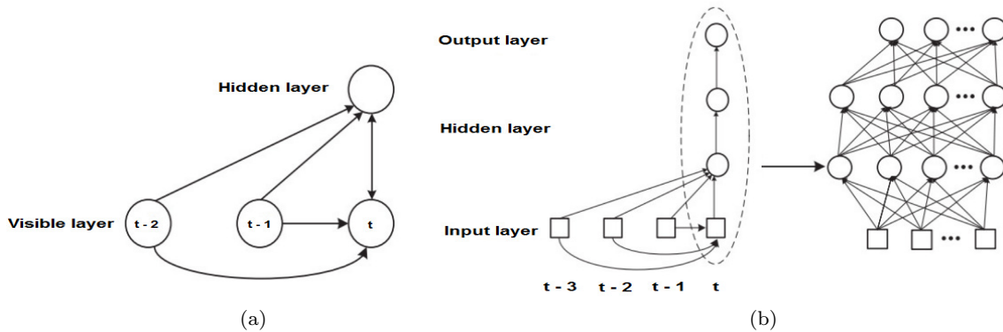
Fig. 24 (a) The cRBM model proposed by Taylor et al. [206]. (b) A modified DBN model designed by Zhang et al. [258].
