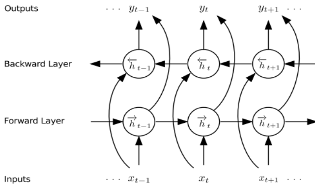
Fig. 13 Architecture of a Bidirectional-LSTM. The circular nodes represent LSTM cells.
