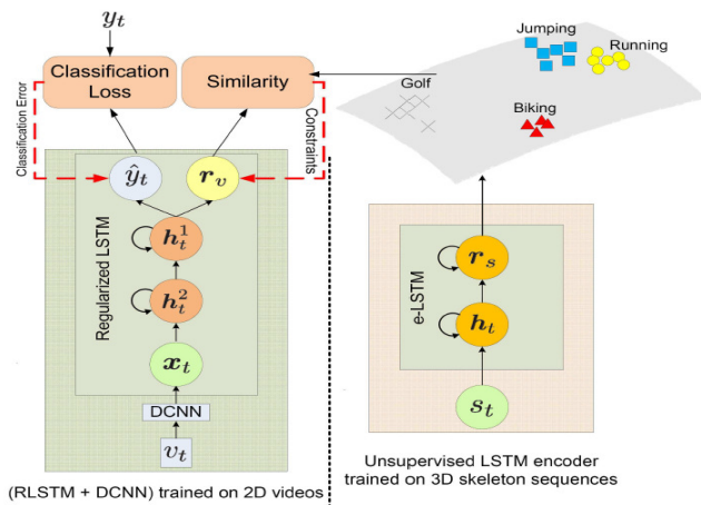
Fig. 23 The parallel DL architecture with RNN-LSTM proposed by Mahasseni et al. [133].
