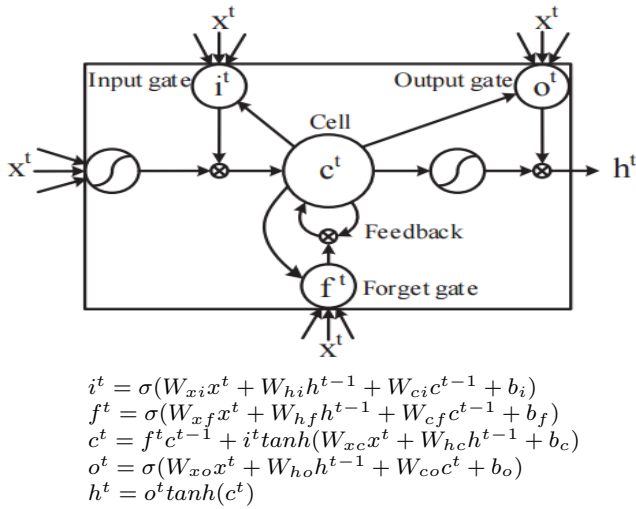
Fig. 12 Diagram of an LSTM unit [62]. A typical LSTM unit contains an input gate i^t , a forget gate f^t , an output gate o^t , an output state h^t and a memory cell state c^t . The information flow is described by the above equations where \sigma is the sigmoid activation; x^t is the input to the network at time t ; all the matrices W are the connection weights between units. \odot denotes element-wise product; and u^t denotes the modulated input function.
