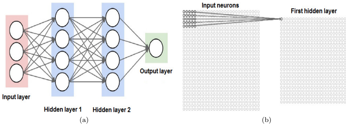
Fig. 8 (a) Illustration of a full-connected model in a regular 3-layer neural network. (b) Illustration of the local receptive field in the input neurons [6].
