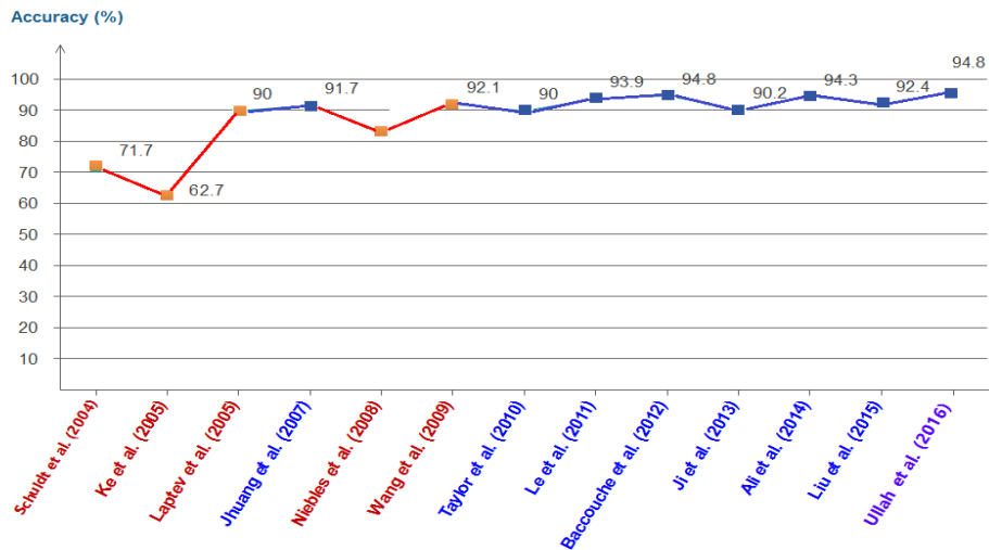
Fig. 29 The recognition performance of hand-crafted and deep learning approaches reported on KTH [173] dataset. The traditional approaches are marked in red. The deep learning based approaches are marked in blue.
