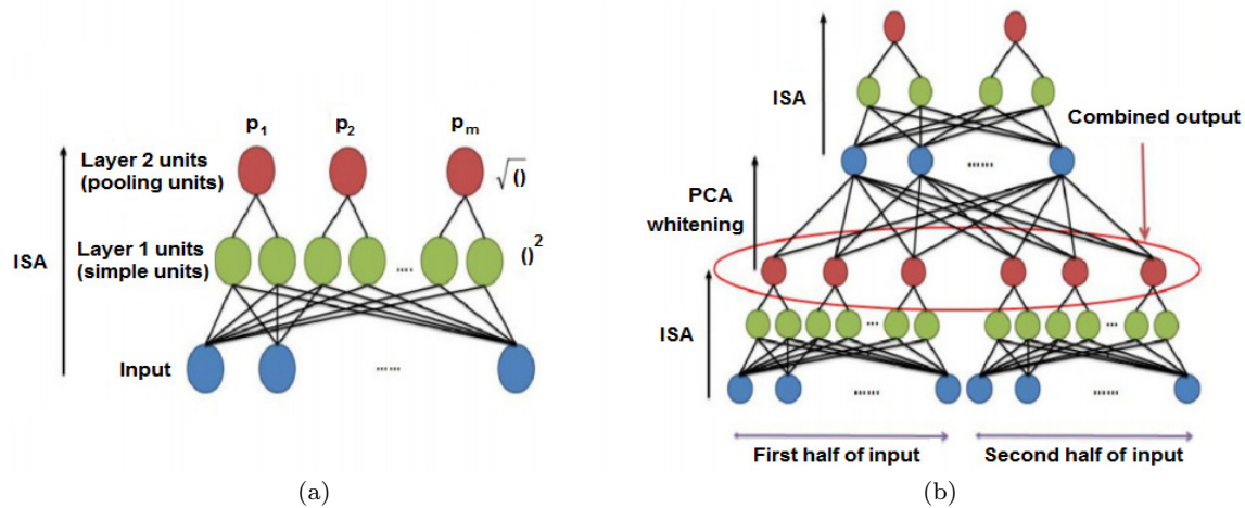
Fig. 27 (a) The structure of an ISA network [114]. (b) Stacking ISA network for building deep architecture [114].
