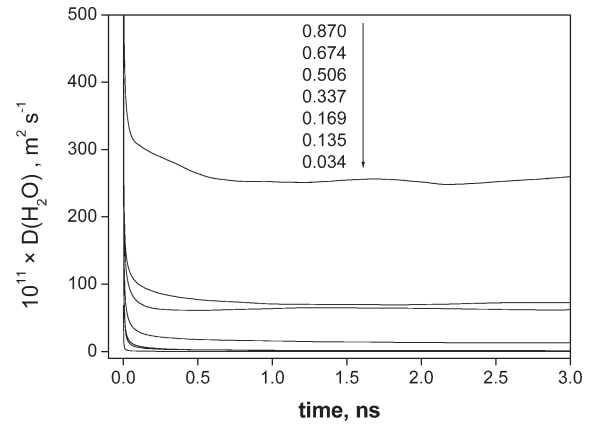
Figure 6. Dependence of the diffusion coefficient of water on time for membranes with different water content that decreases from top to bottom, as indicated in the inset.
