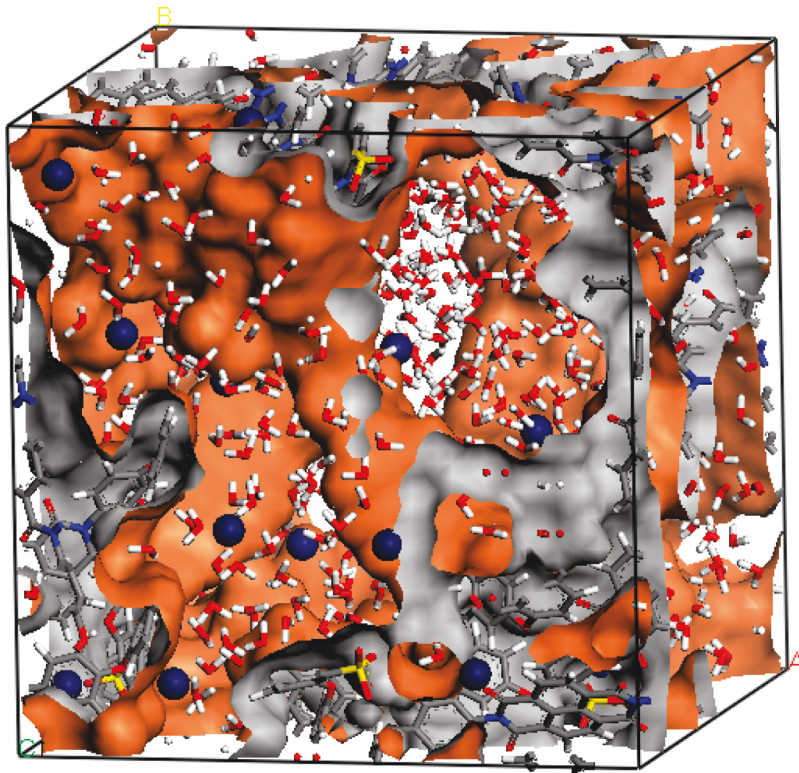
Figure 2. Visual scheme of the fully hydrated MD cell with isosurfaces of polymer chains. Box size: 32.27 Å. Atoms (color): O (red), C (gray), H (white), S (yellow), N (blue), and H + or H 3 O + (blue spheres).
