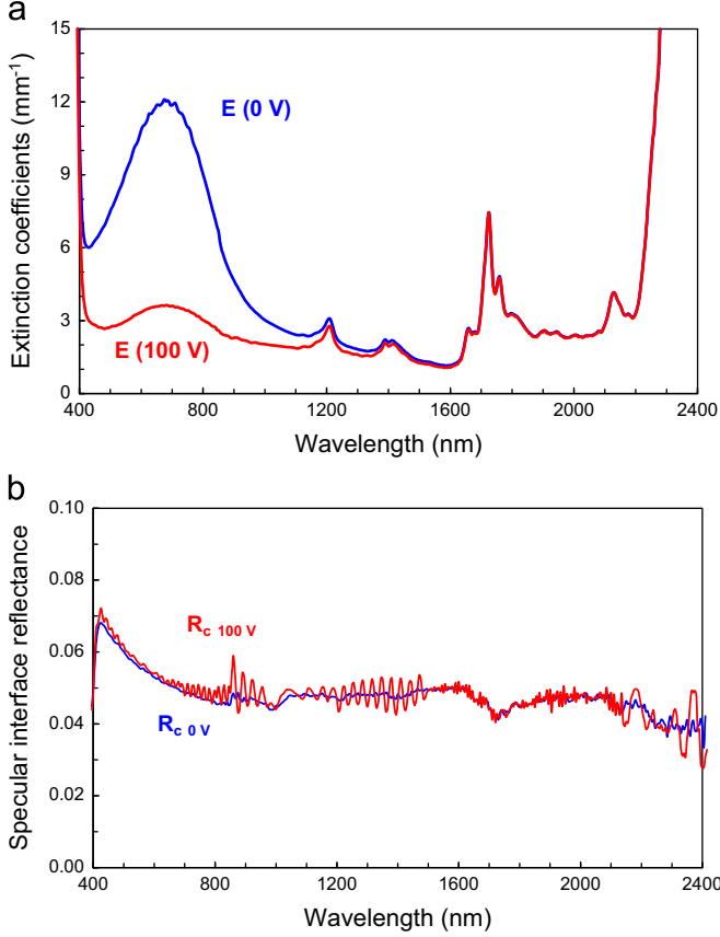
Fig. 8. Spectral extinction coefficient E (panel a) and interface reflectance R_c (panel b) for the SPD at zero voltage (“off” state) and for U=100 V (“on” state).
