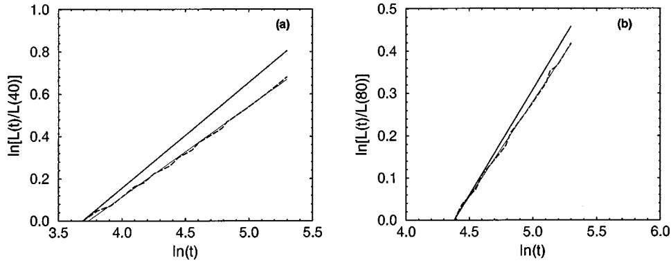
FIG. 4. Solid lines: Analytical values of \ln[L(t)/L(t_{\text{fix}})] for t_{\text{fix}}=40 (a) and t_{\text{fix}}=80 (b). In both cases, \alpha=1 and k_b T=0.6 . Long-dashed lines: numerical values, calculated from Eq. (26). The solid lines over the long-dashed lines correspond to the linear regression of the numerical points.
