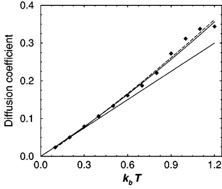
FIG. 2. Lower solid line: the function D_1 ; upper solid line: D_2 , which represent the first- and second-order results for the kink diffusion coefficient [see Eqs. (12) and (23)]. Diamonds represent the numerical values of the kink diffusion coefficient, obtained by numerical integration of Eq. (3) with final time t_f=200 (as in Fig. 1) and different values of k_b T . A quadratic regression of these numerical values is also plotted (long-dashed line).
