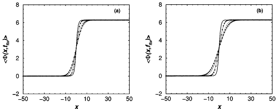
FIG. 3. Solid lines: Snapshots of the evolution of \langle \phi(x, t) \rangle , obtained from numerical simulations of the partial differential equation, for fixed times of 40, 120, and 200, respectively. The initial kink (unperturbed, at rest) is also included for comparison. The width of \langle \phi \rangle increases as time progresses. The superimposed points have been computed numerically from integral (26). Plots correspond to k_b T = 0.4 (a) and 0.8 (b); the width of \langle \phi \rangle is seen to increase also with temperature.
