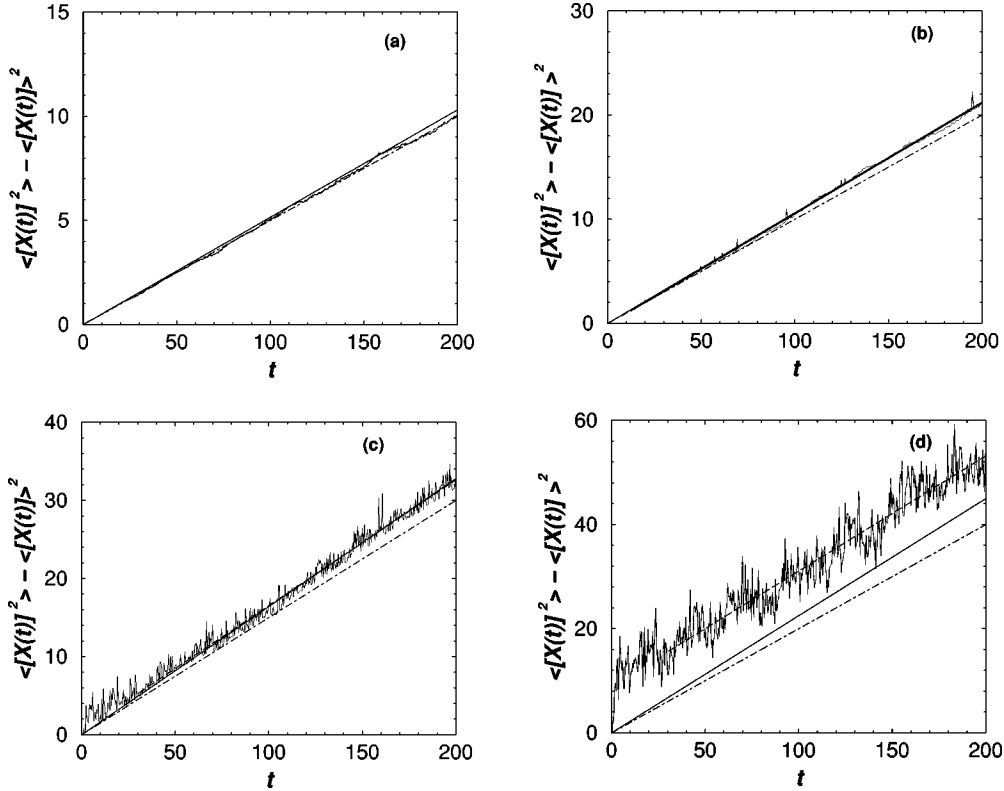
FIG. 1. Simulations with initial condition given by a static kink initially located at X(0)=0 , and subject to a thermal bath. As a continuous (but wiggly) line, we have plotted \langle [X(t)]^2 \rangle - \langle [X(t)] \rangle^2 as obtained by numerical integration of Eq. (3) for (a) k_b T=0.2 , (b) k_b T=0.4 , (c) k_b T=0.6 , and (d) k_b T=0.8 . Superimposed on these lines, the linear regression of the numerical results for t \geq 30 is shown (long-dashed line). The solid line is the theoretical prediction \langle [X(t)]^2 \rangle - \langle [X(t)] \rangle^2 from Eq. (23); this line practically overlaps with the linear regression in (a), (b), and (c). The first-order result \langle [X(t)]^2 \rangle - \langle [X(t)] \rangle^2 from Eq. (12) is shown as a dot-dashed line.
