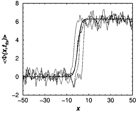
FIG. 5. Average of the wave function for k_b T = 0.4 and t = 200 obtained from 1000 realizations (wider solid line), compared to the average of only five realizations (dot-dashed line). Also represented are three of these individual realizations. Note the different slope and width of the average values as compared to individual realizations.
