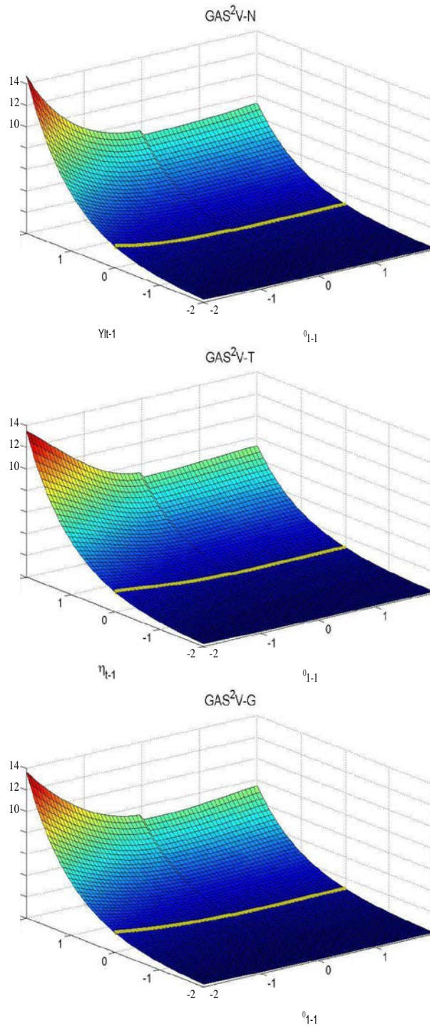
Figure 1: SNIS of GAS 2 V-N (top panel) with parameters (a, cf, k^*, k, u) = (0.07, 0.98, 0.08, 0.1, 0.05) and \exp((1 - cf)u) < 1 , GAS 2 V-T (middle panel) with v_0 = 6 and GAS 2 V-G (bottom panel) with v = 1.5
