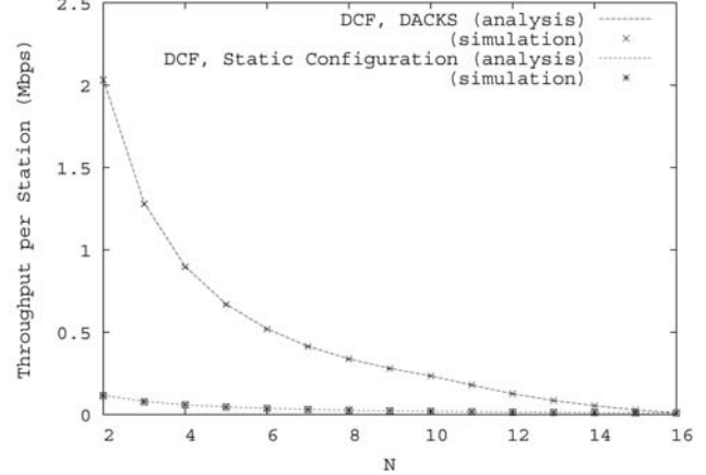
Fig. 12. Inactive stations.
