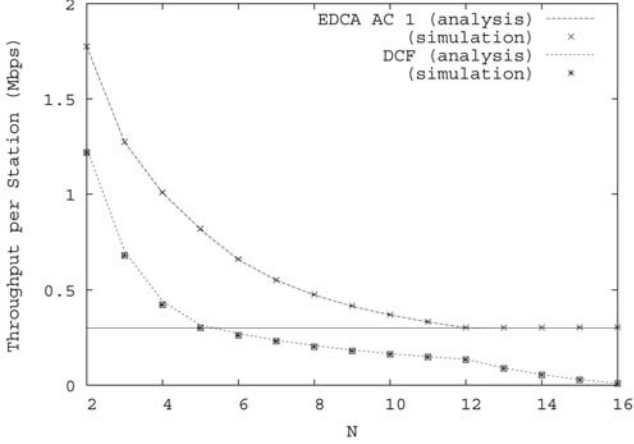
Fig. 5. Throughput guarantees.
