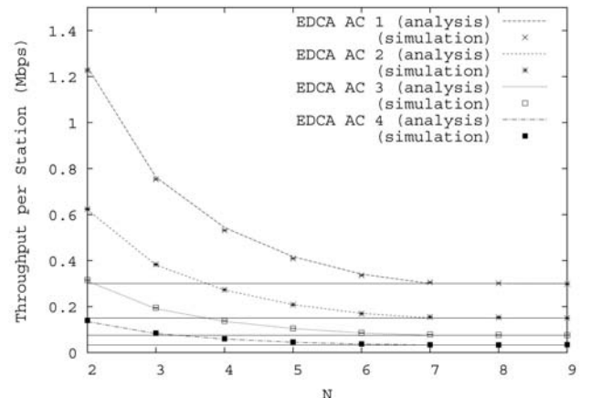
Fig. 13. Multiple ACs.
